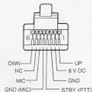
MC-53DM Modular plug (8P)
